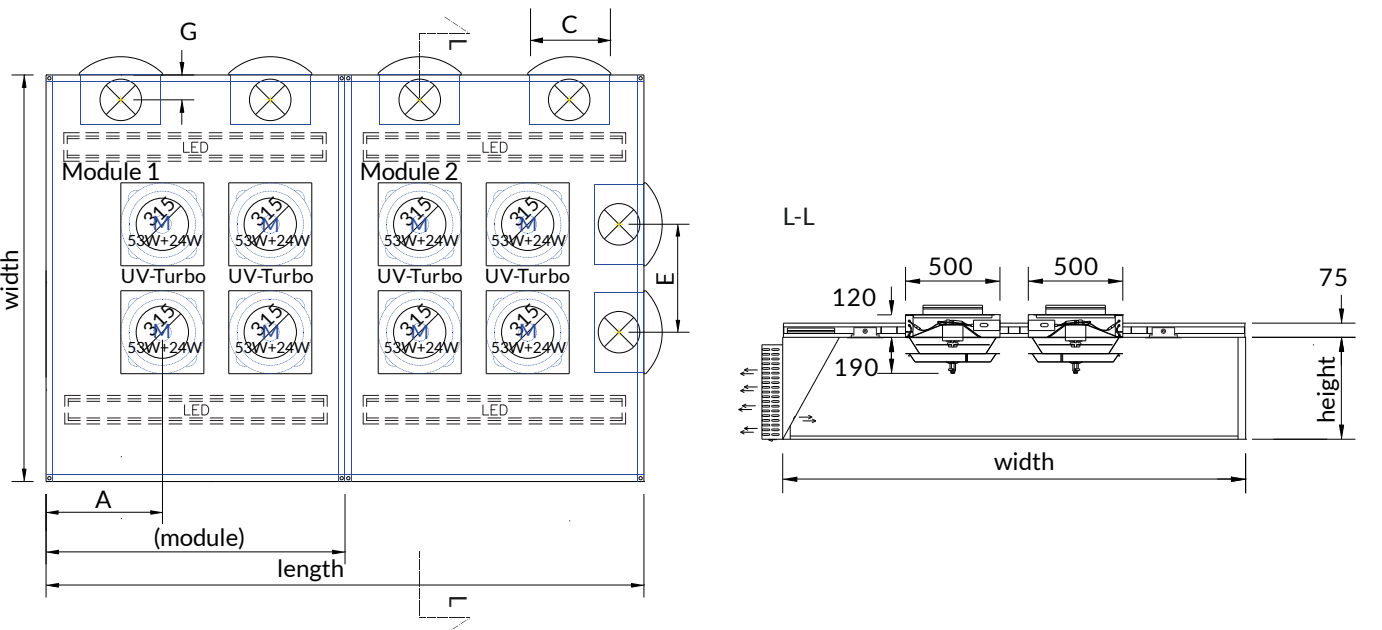
Size and placement of supply air units – supply air hood JSI-R-UV-Turbo
