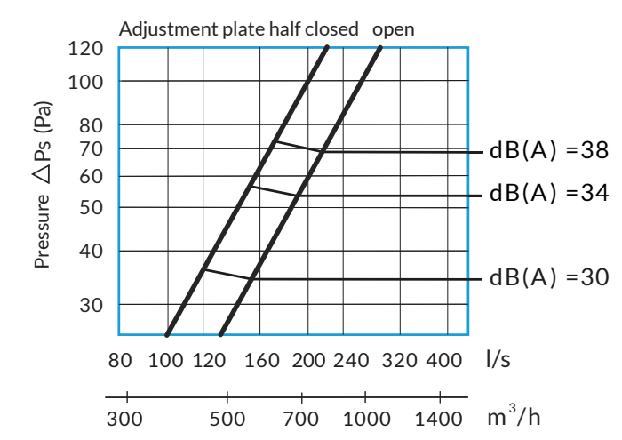
TurboSwing 750 rpm
