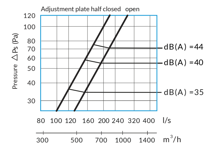
TurboSwing 1100 rpm
